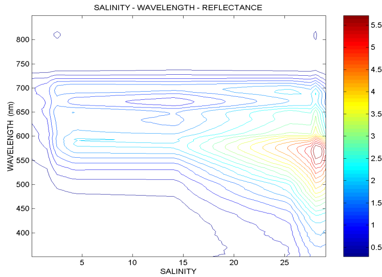
Figure 3: Spectral response in the test site as a function of salinity and reflectance based on the stations shown in Figure 1. The colour bar represents the code for isolines of reflectance R(\lambda) in percent. Data were collected on a cruise in 2001.
