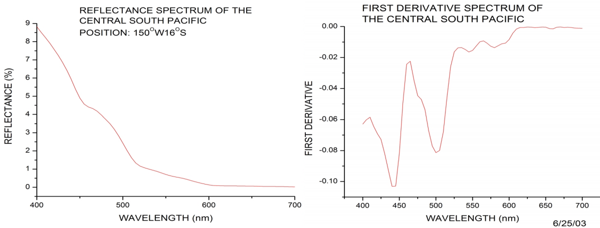
Figure 5: Reflectance [R(\lambda)] spectrum of clear ocean water (left) and first derivative (right). The raw data were provided by Dr. S. Maritorea, University of California.
