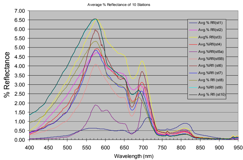
Figure 4: Averaged subsurface irradiance reflectance [R(\lambda)] spectra through the salinity gradient based on data collected on a cruise in 2002.
